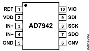
Figure 4.10-Lead MSOP and QFN (LFCSP) Pin Configuration
