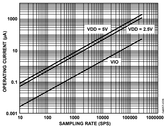
Figure 28. Operating Currents vs. Sampling Rate
